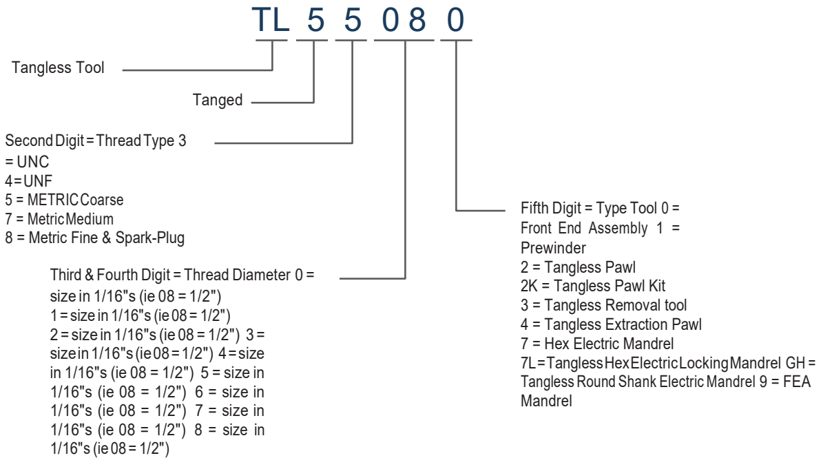
Example-Tangless M8-1.25 Front end assembly
